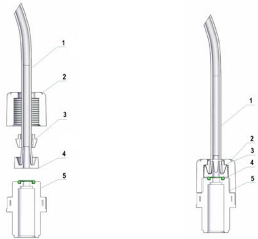
Fig.4 – Tubes connection
