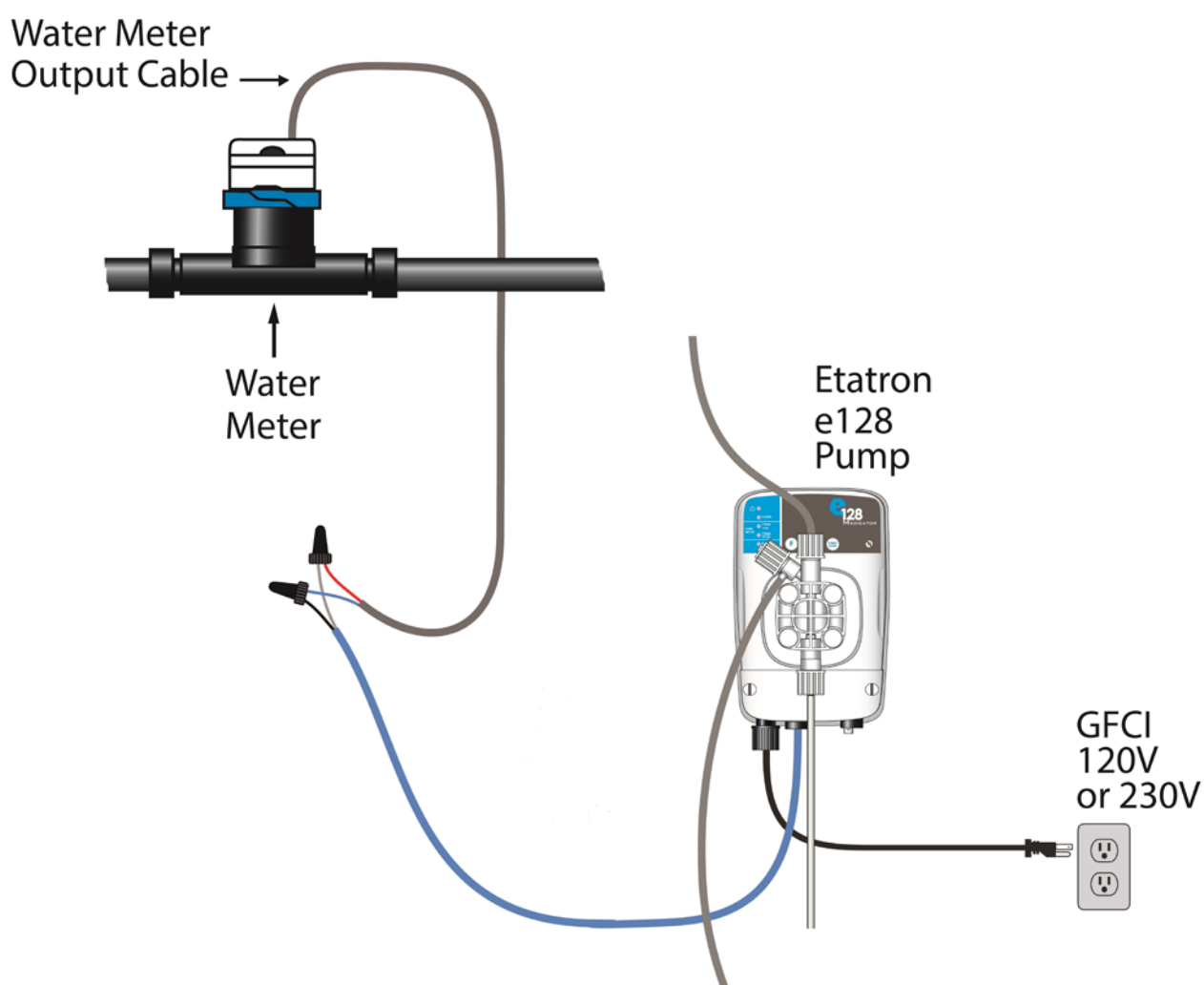
Fig. 9 – Water meter connections
