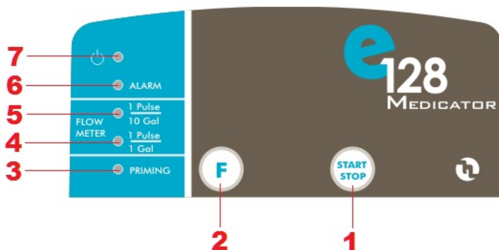
Fig.8 - Commands panel
