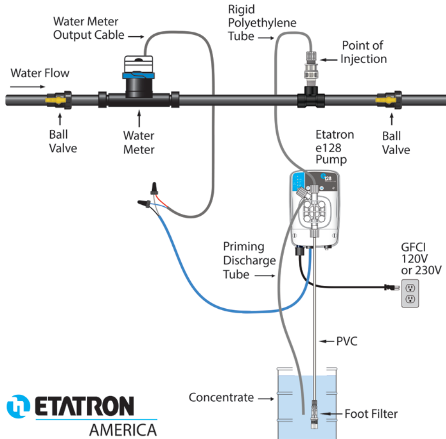
Fig. 6 – Typical installation
